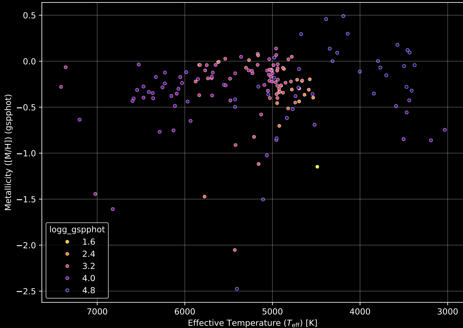
APOGEE DR17 Field: [058+57] Stellar Population Parameters (n= 161)
