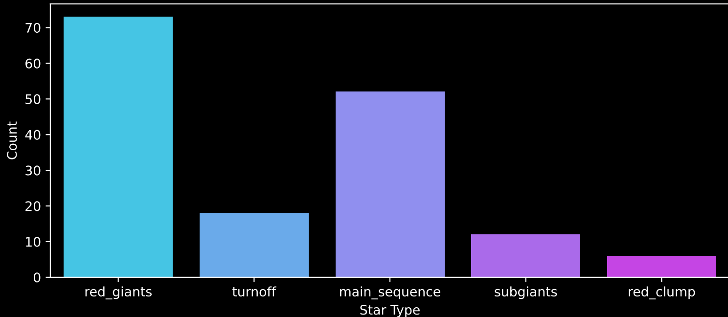
APOGEE DR17 Field: [058+57] Count plot of Star Type
