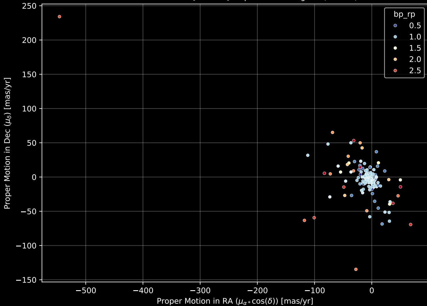
APOGEE DR17 Field: [058+57] Proper Motion Diagram (n= 161)
