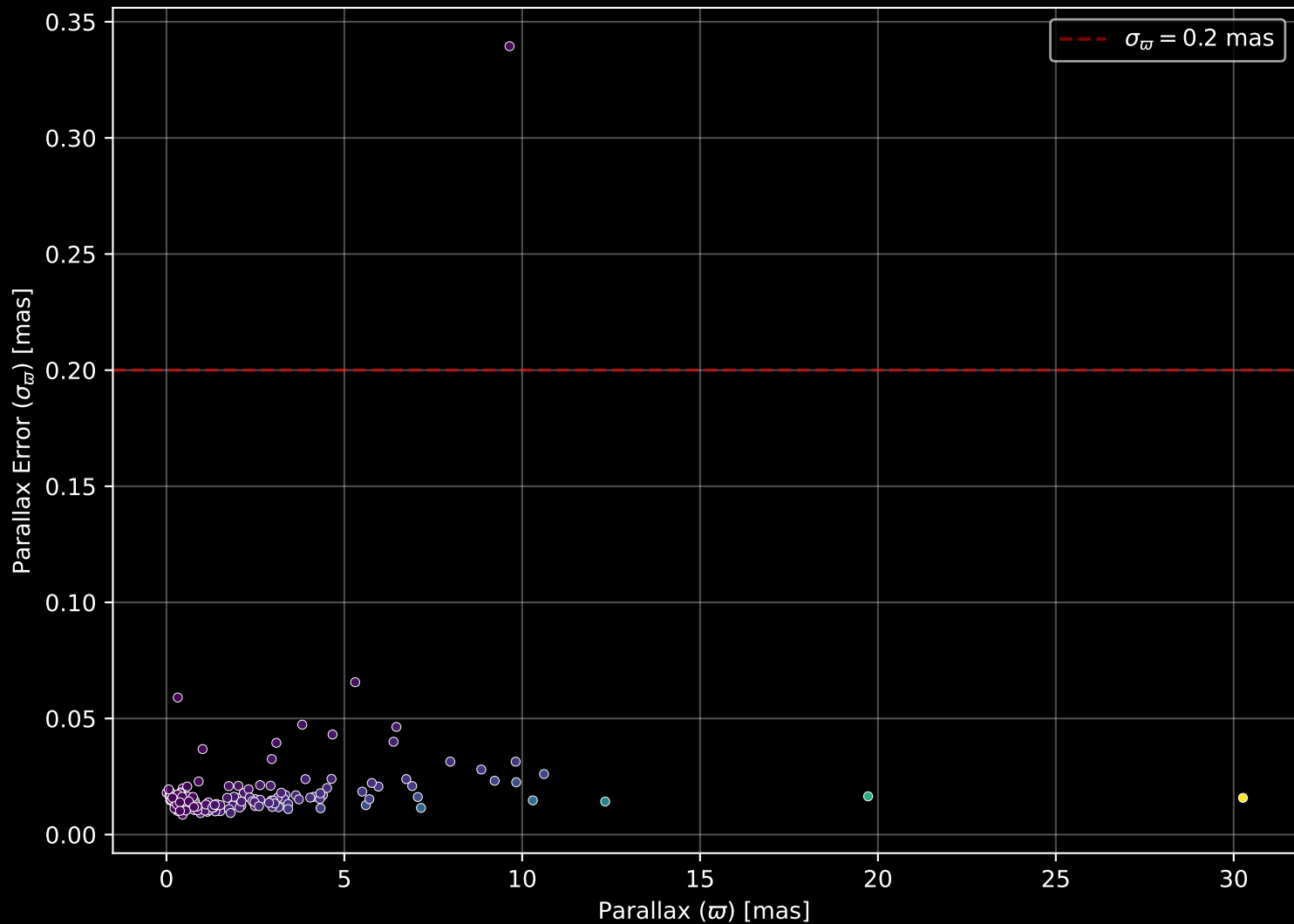
APOGEE DR17 Field: [058+57] Parallax Quality (n= 161)
