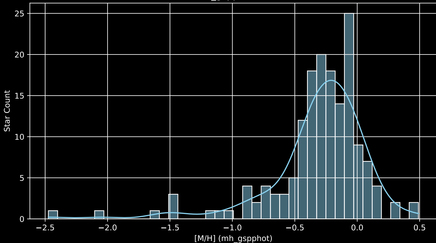
APOGEE DR17 Field: [058+57 [M/H] (mh_gspphot) (n= 161)
