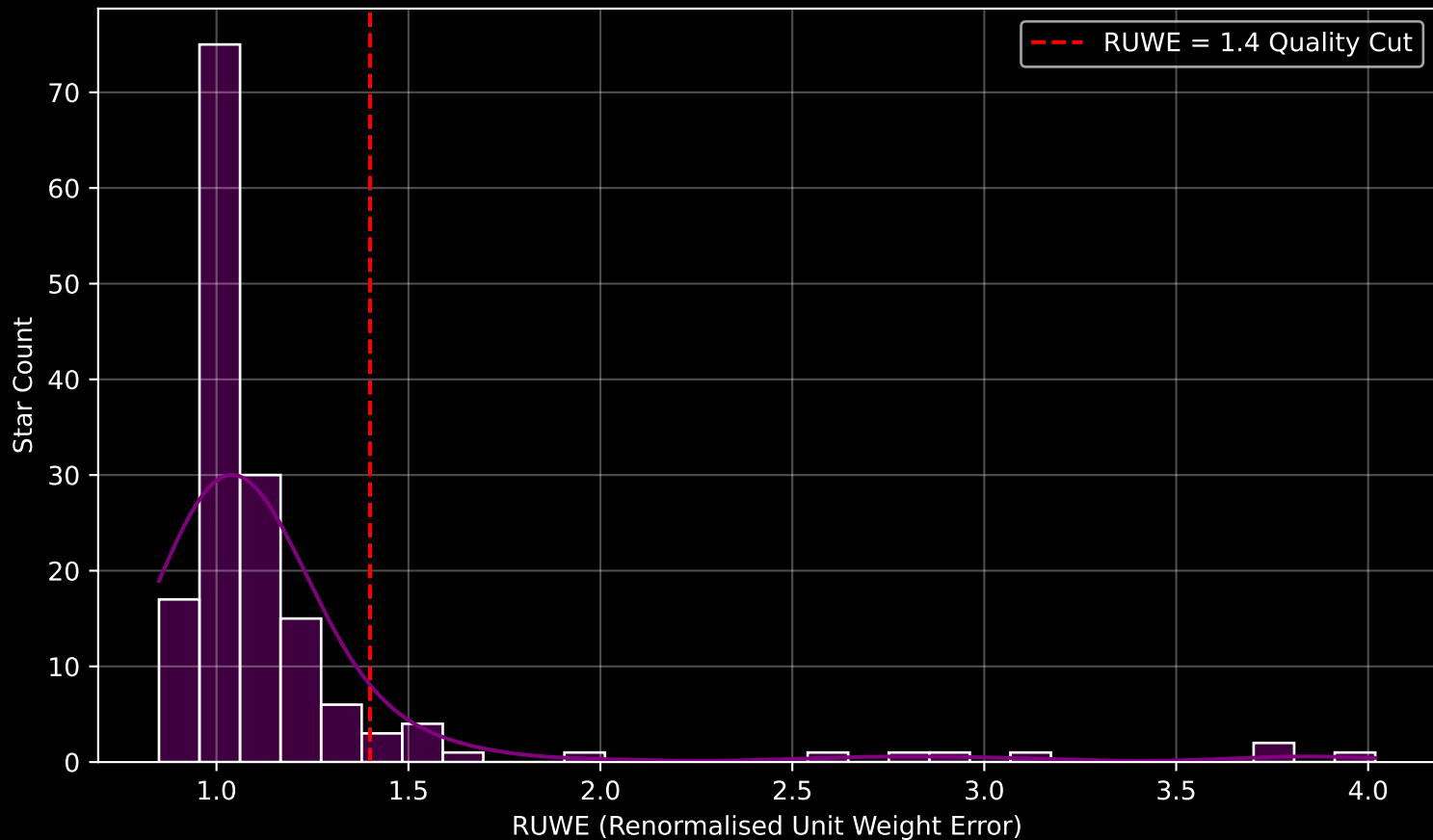
GAPOGEE DR17 Field [058+57] RUWE Distribution (n= 159)
